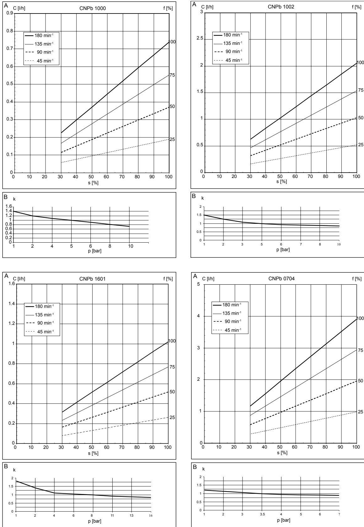
Fig. 1: A) Capacity C for medium back pressure dependent on the stroke length s for different stroke rates f. B) Corresponding correction factors k dependent on back pressure p.
