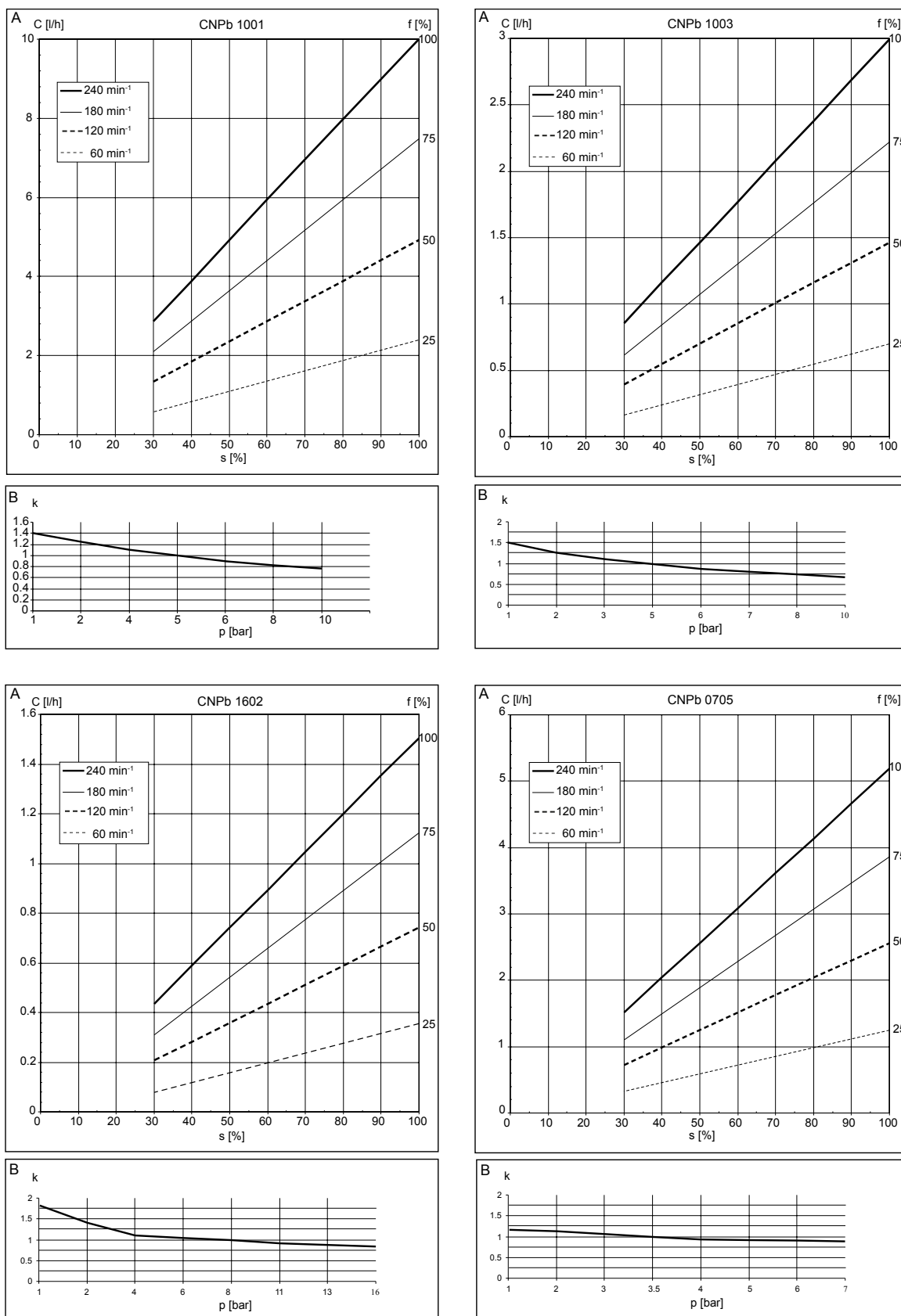
Fig. 3: A) Capacity C for medium back pressure dependent on the stroke length s for different stroke rates f . B) Corresponding correction factors k dependent on back pressure p .
